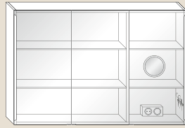
SPES/SPEW L/R H 800 x T 170-200 x B 1100, 1200, 1300, 1400, 1500 mm
