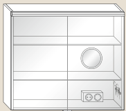
SPQK/SPQL H 700 x T 170 x B 600, 800, 900, 1000 mm
