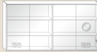
SPES/SPEW H 800 x T 170-200 x B 1600 mm
