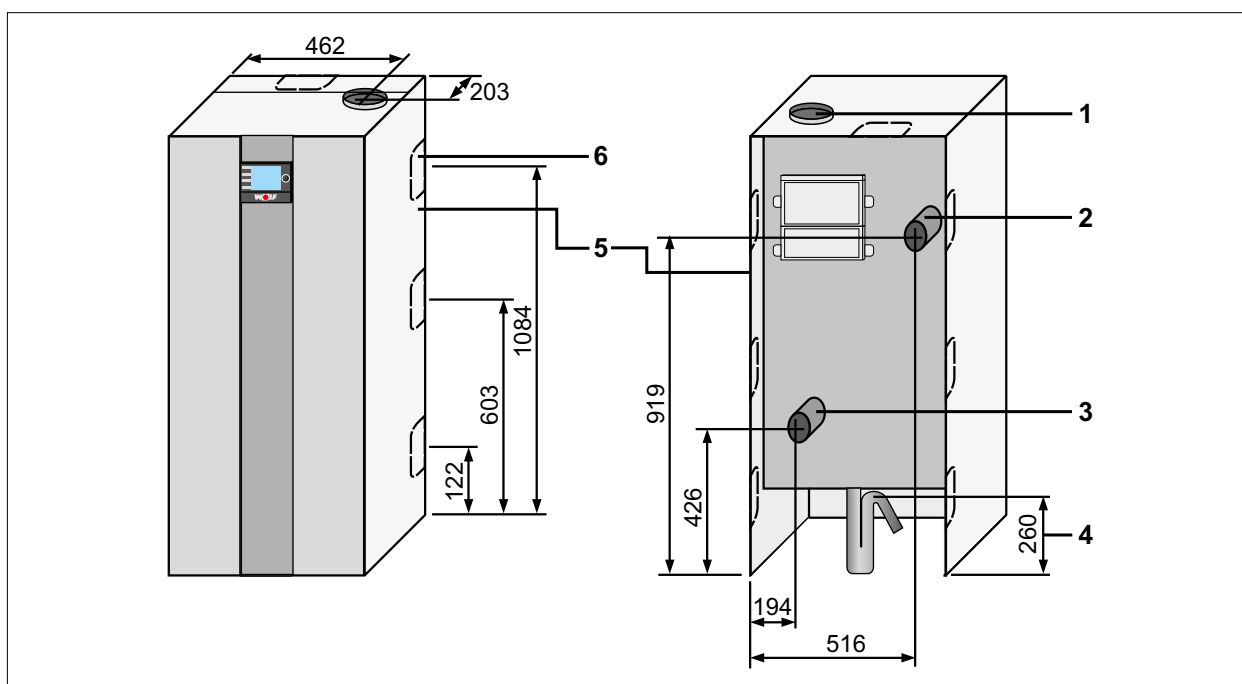
Abb. 12.4 Anschlüsse COB [mm]
