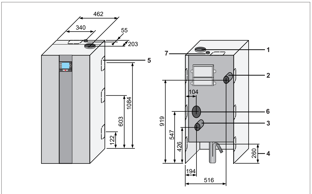
Abb. 13.4 Anschlüsse TGB-2 [mm]
