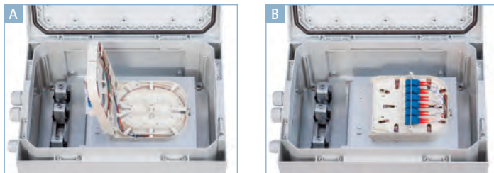
Hinged splice cassette for easy assembly
