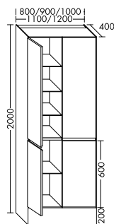
SGJB080/090/100/110/120
