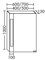
SPNK040/050/060/070 SPOG040/050/060/070*
