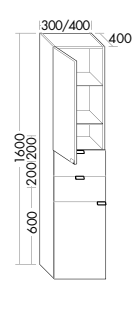
HSMU030/040
