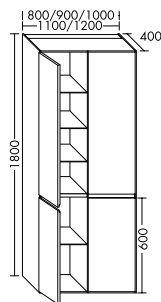
SGJD080/090/100/110/120
