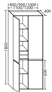
SGJE080/090/100/110/120
