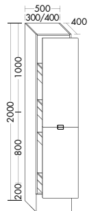
HSQN030/040/050
