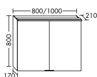
SPMV080/100 SPNR080/100*
