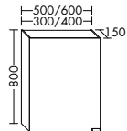
SPNI030/040/050/060 SPOE030/040/050/060*
