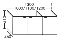
WWOD100/110/120/130
