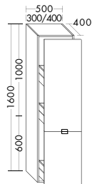
HSQP030/040/050
