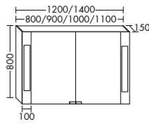
SPNH080/090/100/110/120/140 SPOD080/090/100/110/120/140*
