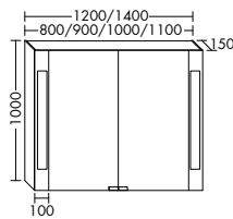
SPNM080/090/100/110/120/140 SPOI080/090/100/110/120/140*
