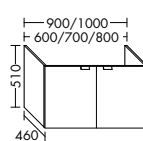
WWOC060/070/080/090/100
