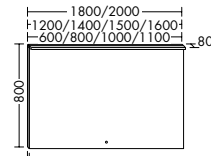
SIJA060/080/100/110/120 SIJA140/150/160/180/200
