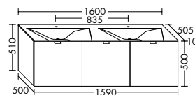
SFYA160
