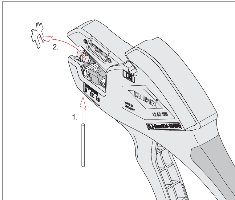
Removing the bottom blade
