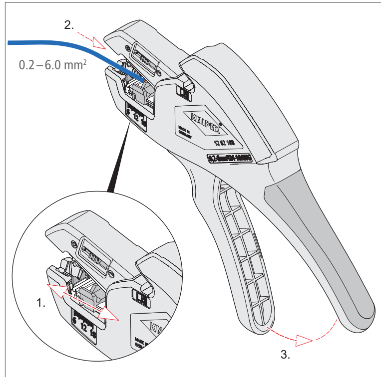
Stripping single conductors
