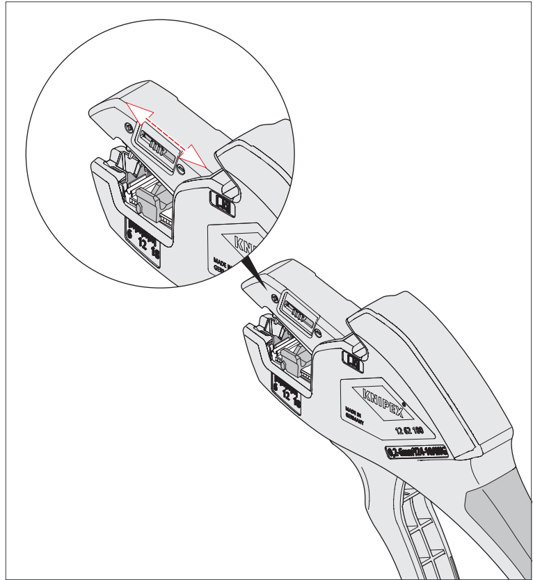
Readjusting the cutting depth
