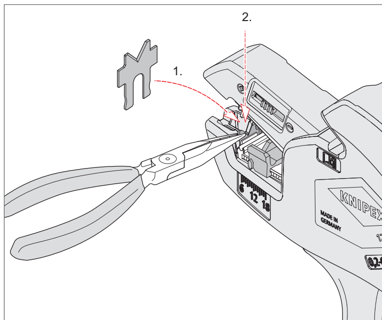
Installing the bottom blade
