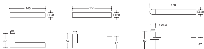
Model 101X | 101XPH
