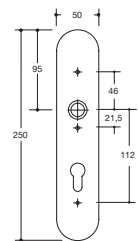
Schild 235.21X..
