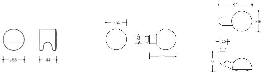
Knopf 122.23
