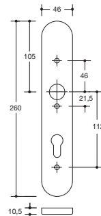
Schild 235...
