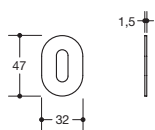
Schlüsselrosette 306P..M..
