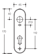
Schild 230...X..
