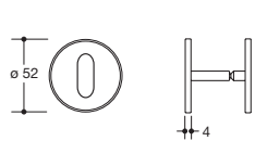
Schlüsselrosette 306.23..I..
