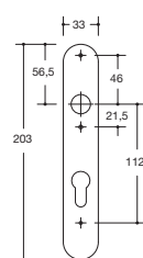
Schild 219.21X..H
