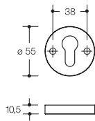
Schlüsselrosette 306X.23X..
