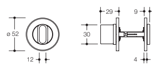
WC-Rosette 306..INRHT
