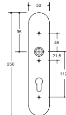
Schild 235.21X..
