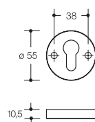
Schlüsselrosette 306X.23X..
