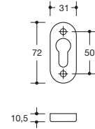
Schlüsselrosette 316...
