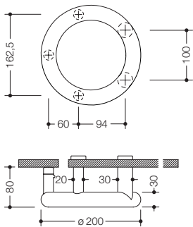
HEWI Griff ø 30 mm
