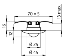
sensor head
