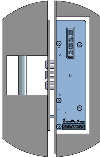
Detail Z 1:2 FTV 320
