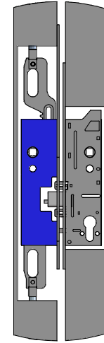
Detail X 1:5 IQ lock DL 9235
