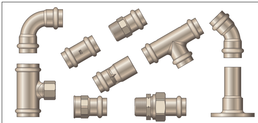
Fig. 1: Seapress – Overview
